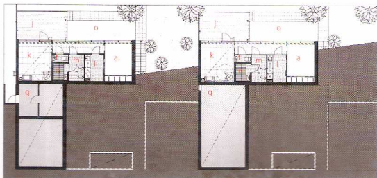
1:200 pohjakerros / 1st floor
